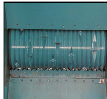
Rotor Cutter Made From Hardened Tool Steel
